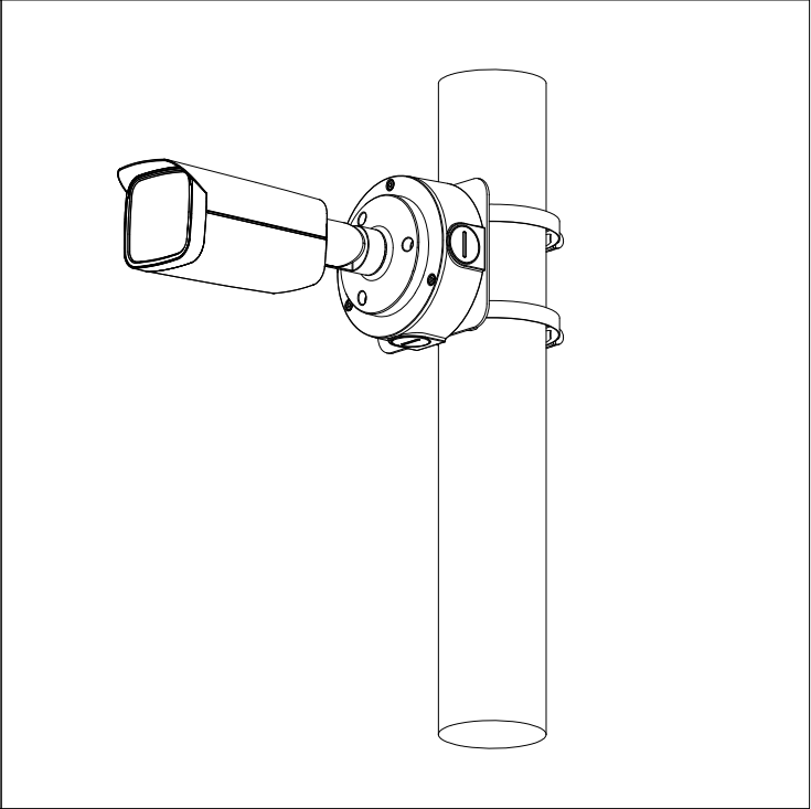
Pole Mount(Vertical)
