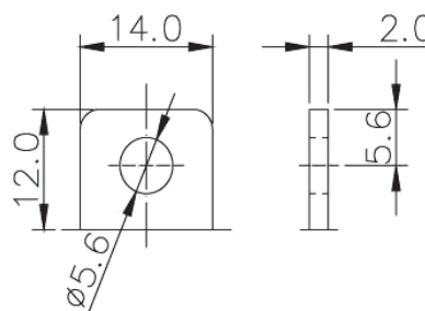
Terminal Type (mm)
