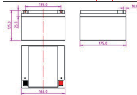
Outer dimensions (mm)
