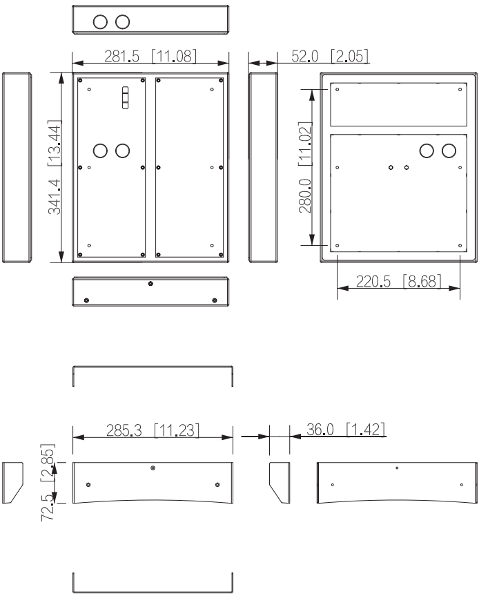
Dimensions (mm[inch])
